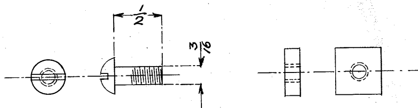
STANDARD STOVE BOLT AND NUT
